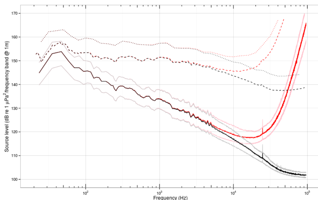
Figure 4. Source level ( SL ) spectra of the entire ship population in 1 Hz (solid), 1/12-octave (dashed), and 1/3-octave bands (dotted). Black curves are medians without absorption; red curves are medians with absorption. For the spectrum levels, we delineate 25 and 75% quantiles in lighter tones. Levels with-absorption which go off-scale for the 1/12- and 1/3-octave bands are 195 and 202 dB, respectively, at 96,000 Hz.
