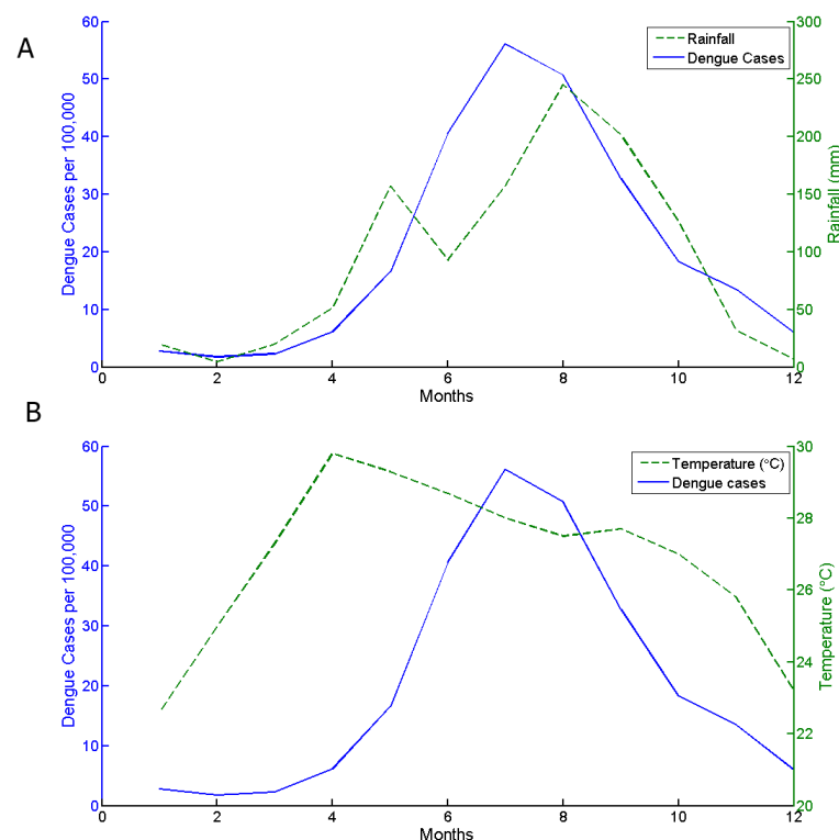
Figure 1: The average monthly incidence rate of dengue during 2009–2015 in Chiang Mai, Thailand is indicated by the complete line.
