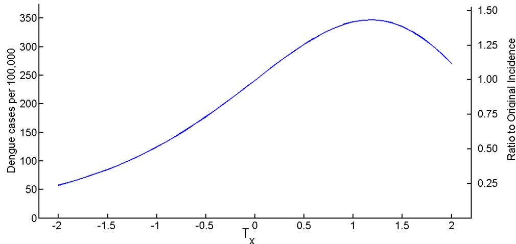
Figure 5: The number of total incidences in one year as the temperature changes ( T_x ) from the mean temperature of Chiang Mai during 2009–2015 ( T_x = 0 ).
