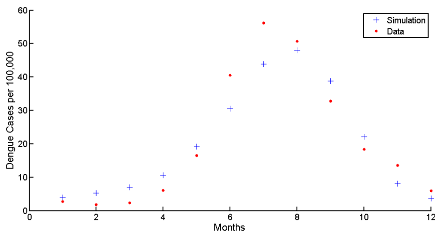
Figure 2: The number of monthly dengue incidences generated by the model and actual data of Chiang Mai from 2009 to 2015.
