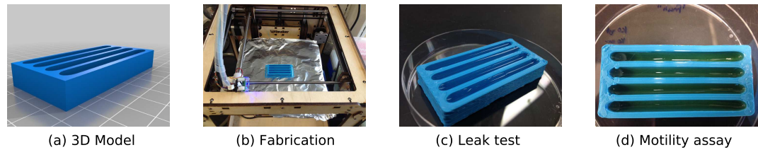
Figure 4. A custom device for a motility assay fabricated using 3D printing. The device was found to be sterile without autoclaving if contamination during post-fabrication handling is avoided.
