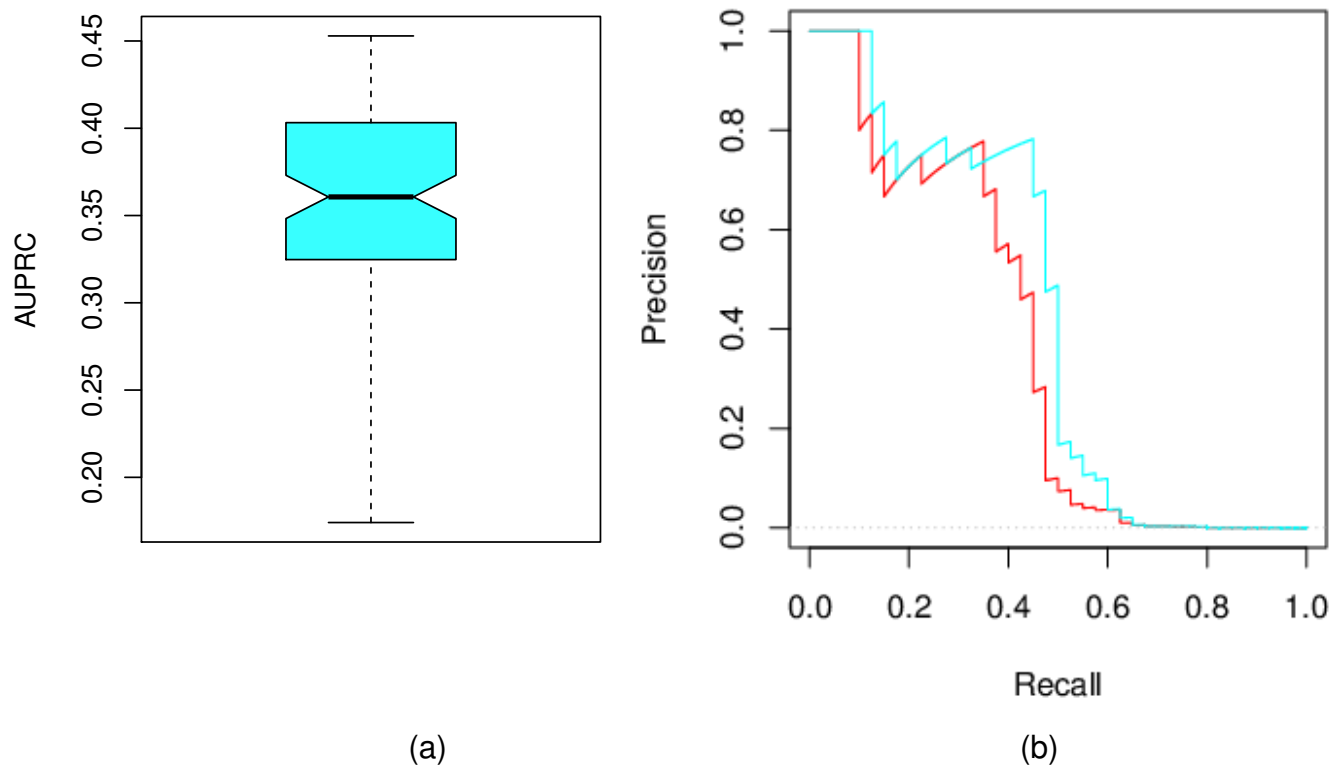
Figure 1: (a): Distribution across 100 different choices of hyperSMURF parameters ( n, f, m ) of the AUPRC values obtained by cross-validation on the training data; (b) Comparison of precision-recall curves obtained by hyperSMURF with default parameters (red curve) and with the selected “best” parameters (cyan curve).
