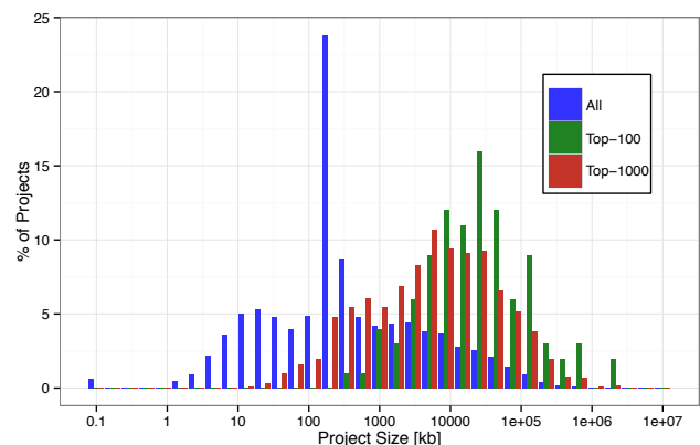
Fig. 3. Distribution of project sizes
