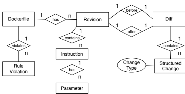
Fig. 2. Relational data model to support queries for data analysis.
