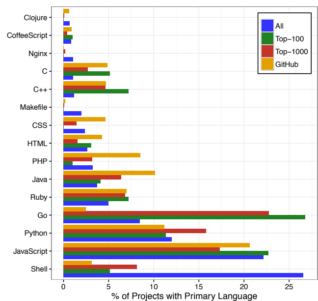
Fig. 4. Distribution of top 15 languages in our dataset
