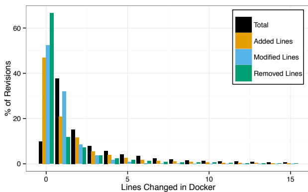
Fig. 9. Distribution of revision sizes measured in lines changed
