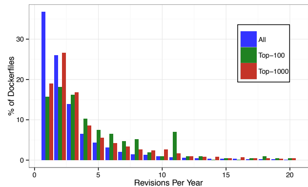
Fig. 8. Distribution of yearly revisions
