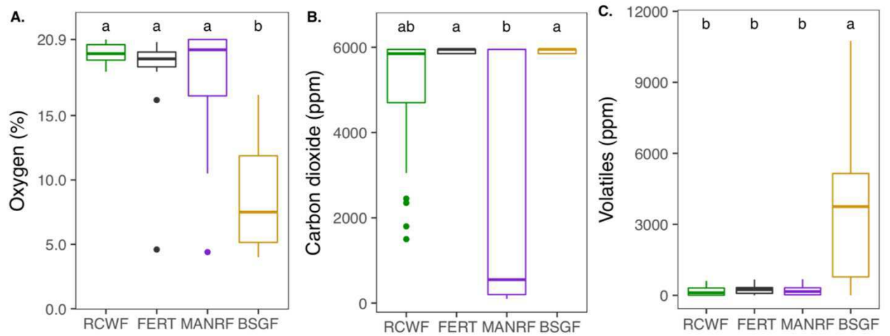
Figure 3. Gas concentrations in the center of the treatment bins measured seven times over 45 days.
