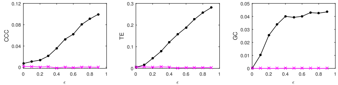
Figure 4. (color online). Causality estimated using CCC, TE and GC for coupled AR(1) processes, from Y to X (solid line-circles, black) and X to Y (solid line-crosses, magenta) as the degree of coupling, \epsilon is varied. CCC, TE as well as GC are able to correctly quantify causality.
