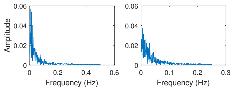
Figure 9. Frequency Spectrum of dependent AR(1) process from Set 1 without decimation (left) and when decimation factor equals 0.5 (right). The process does not undergo aliasing on decimation.
