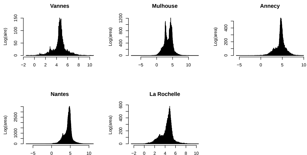
Figure 2. Histograms of log-transformed data
