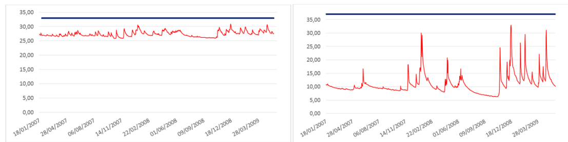
Figure 5. Example of phreatic table variations in time observed in two neighboring piezometers; the red and blues lines indicates the heights of water table and of ground surface with respect to bedrock respectively.
