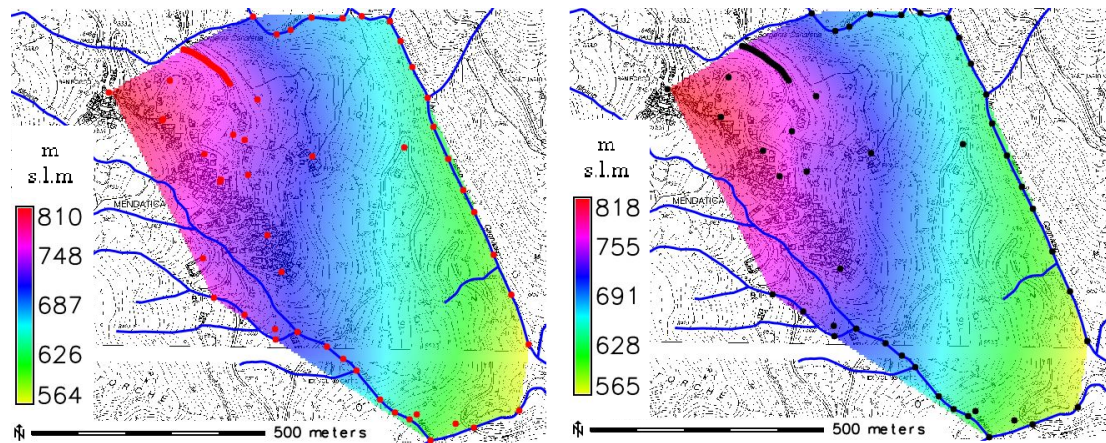
Figure 1. Digital model of the bedrock (left) and of the average groundwater table (right). The red dots represent the boreholes or emerging rock locations, the black ones show piezometers or wet riverbeds locations.
