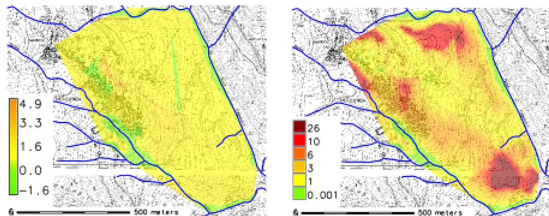
Figure 6. Groundwater level variations (in m) evaluated by r.gwflow (left) and IHG model (right).
