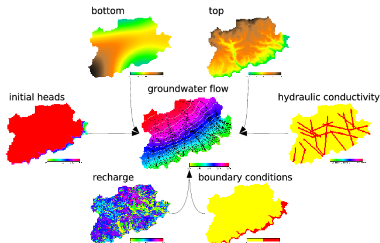
Figure 2. Workflow of r.gwflow .
