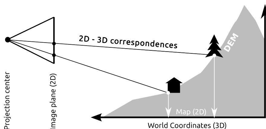
Figure 1. Perspective geometry: the camera orientation is computed from 2D-3D correspondences.
