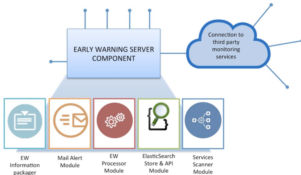
Figure 2. The Server Components of the HELP EW System.
