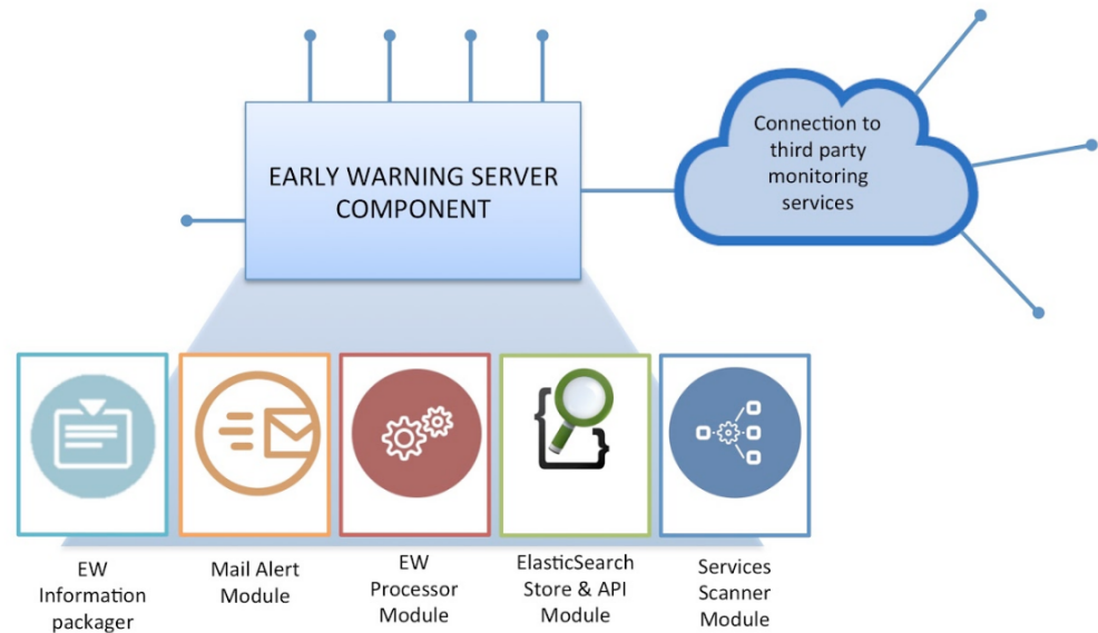
Figure 2. The Server Componets of the HELP EW System.
