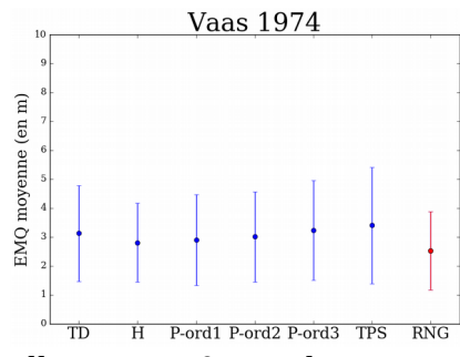
Illustration 10: Results on Vaas 1974 data
