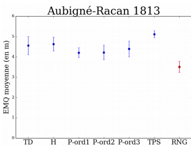
Illustration 5: Results on Aubigné-Racan 1813 data
