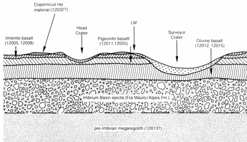
Figure 1: Apollo 12 Landing site cross-section [Harland, 2008]
