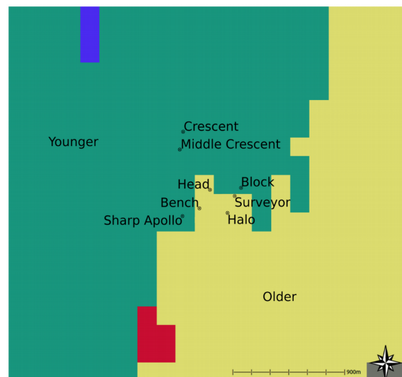
Figure 5: M 3 image segmentation in close proximity of the landing site
