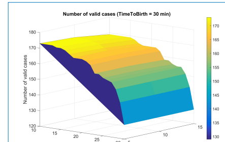
Figure 5: Result of CAPIM selection process. This plot displays the number of valid cases as a function of selection parameters T_{SUM\_min} and T_{CTG\_min} . Further Parameters are pH_{umbilical} < 7.1 and TimeToBirth = 30 min. The dataset is from the Frauenklinik und Poliklinik, Technische Universität München, Munich, Germany. It describes the time frame between 09/2009 and 12/2015. The total number of possible cases with pH < 7.1 was n = 477 . The lower number of valid cases is caused by inappropriate CTG files and/or exclusion of primary caesarian sections.
