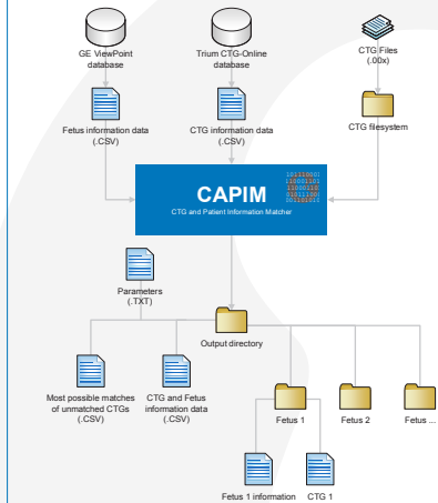
Figure 2: Information flow of „CTG And Patient Information Matcher“ (CAPIM). CAPIM gets information about fetus, all CTGs and additionally the path where the CTG-Files are stored. Furthermore a directory structure with all selected and valid CTG files and files with relevant information for further processing will be created.
