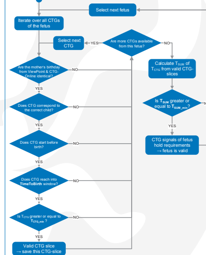
Figure 4: Flowchart of the CAPIM selection process to select only cases, which hold the defined requirements ( T_{TimeToBirth} , T_{CTG\_min} , T_{SUM\_min} ).
