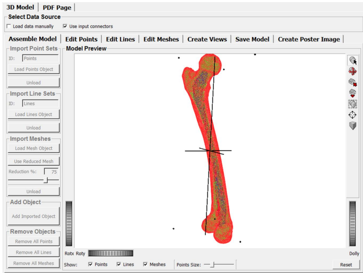
249 250 Figure 2. User interface of the app. The user interface comprises all necessary steps for the creation of 251 3D model files and PDF files. It is arranged in tabs for each step.
