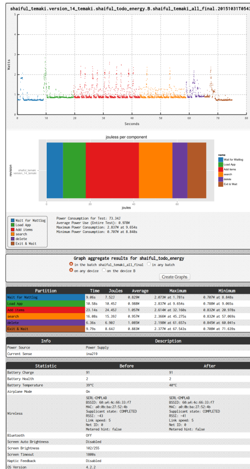
Figure 2. Green Miner Example Test Run
