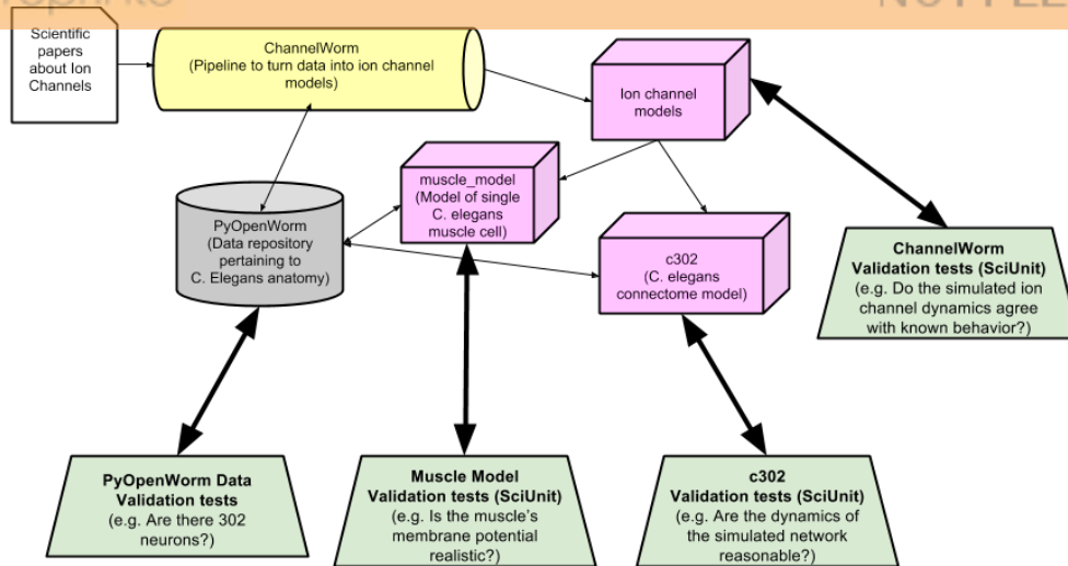
Figure 1. Diagram of the some key OpenWorm modules and their corresponding testing frameworks.
