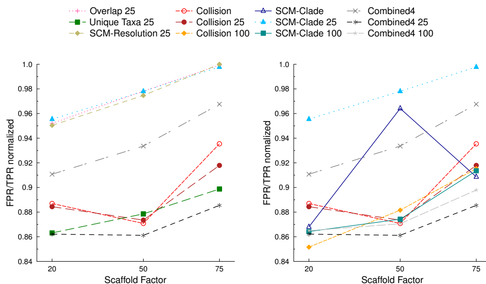
Figure 4. Left: \frac{FPR}{TPR} for the different scorings with and without randomization for the different scaffold factors (20%, 50%, 75%) on the 500 taxa dataset. The values are normalized per scaffold factor. Combined4 is the semi strict consensus of the supertrees calculated by Collision, Unique Taxa, SCM-Resolution and the SCM-Clade scoring. The integer value behind scoring names represents the number of randomized iterations
