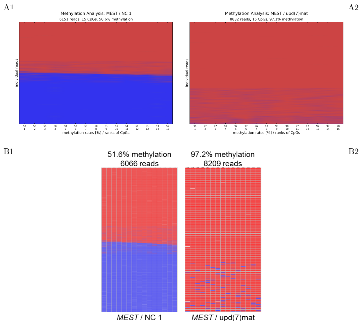
Figure 2: Methylation analysis of the imprinted MEST locus on human chromosome 7q32 by (A) amplifyer and (B) BiQ Analyzer HT . In individual methylation plots, each row corresponds to an individual read and each column to a CpG. A red rectangle represents a methylated CpG, a blue rectangle an unmethylated CpG. Plots A1 and B1 show the methylation status of individual reads of a normal control (NC). The overall average methylation is approximately 50%, as expected for an imprinted locus. The reads can be separated into reads from the methylated maternal allele and reads from the unmethylated paternal allele. Plots A2 and B2 show an individual with hypermethylation for this locus. This hypermethylation is caused by a maternal uniparental disomy for chromosome 7 (upd(7)mat), i.e., the presence of two methylated maternal chromosomes 7 and the absence of an unmethylated paternal copy for chromosome 7.
