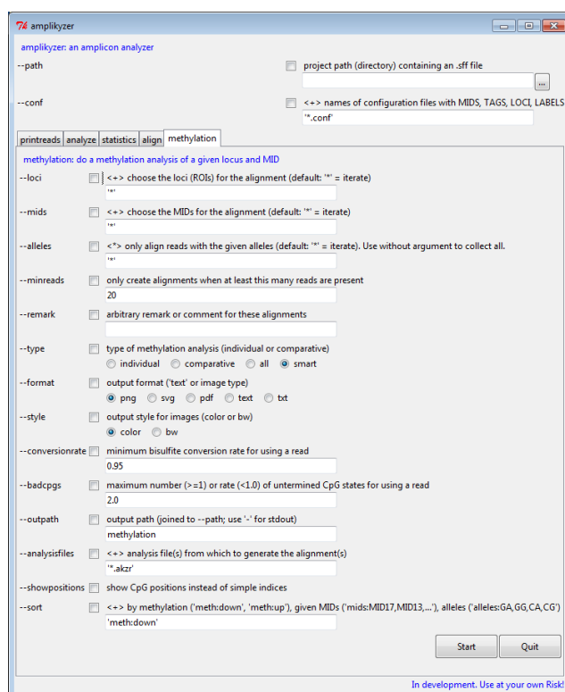
Figure 8: Part of the graphical user interface (GUI) of amplykizer, showing the options for methylation analysis.
