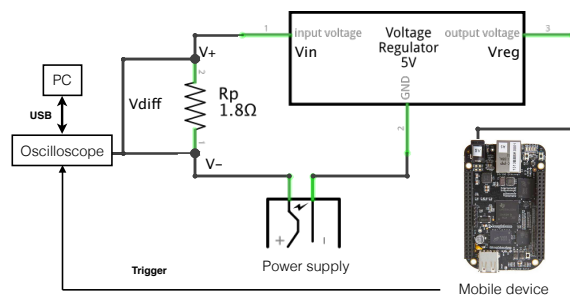
Fig. 1. Measurement setup.
