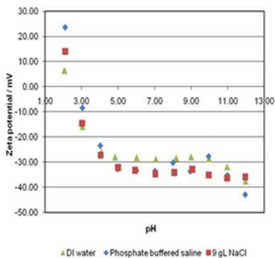
Fig 1: Effect of different wash buffers on zeta potential-pH profiles of E. coli grown in LB Lennox (with 2 g/L glucose). Larger version of the figure is in the supplementary information.
