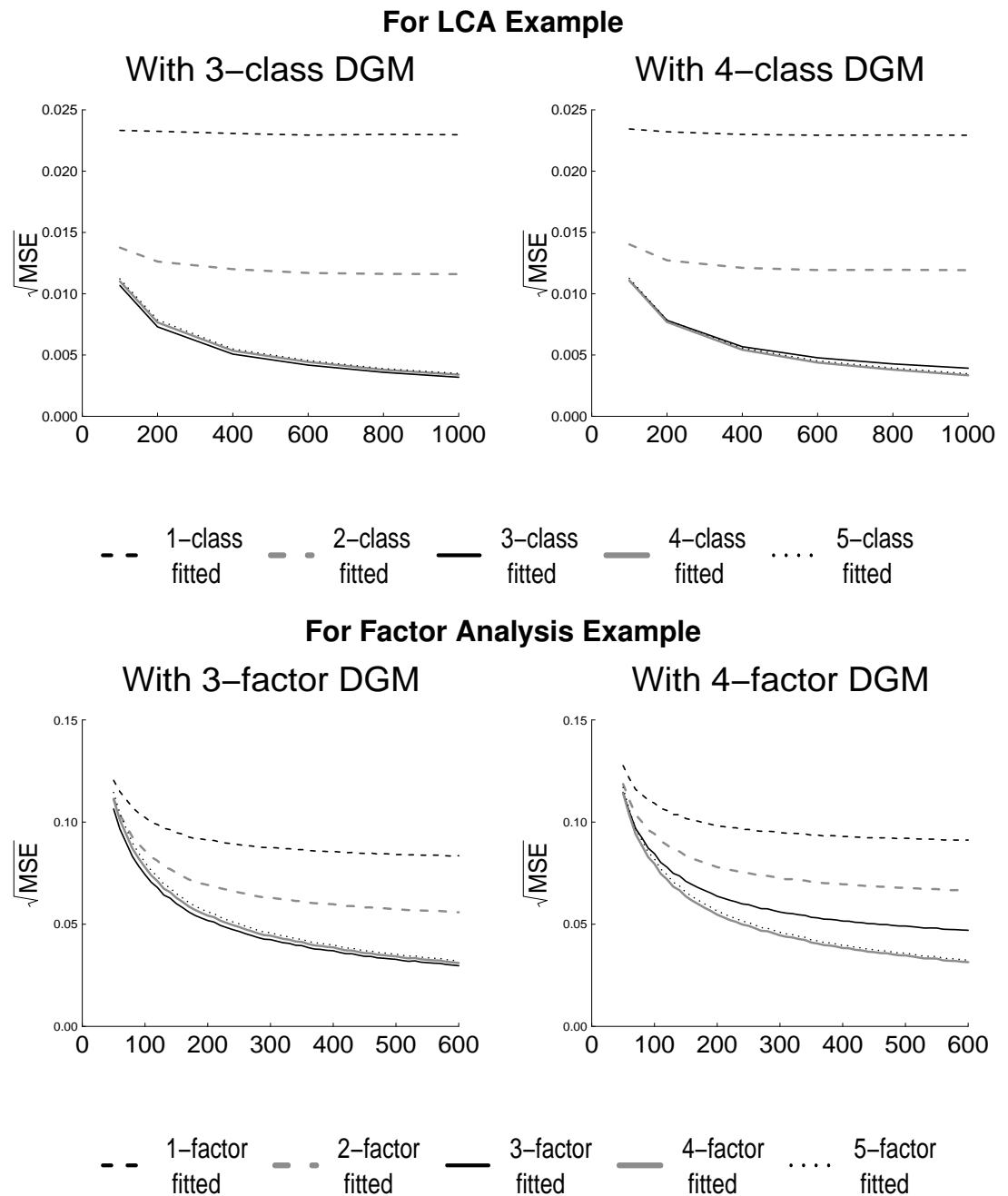
Figure 5. Estimation performance by models of various fixed sizes in the LCA and factor analysis examples. “DGM” denotes data-generating model (simulated true model).
