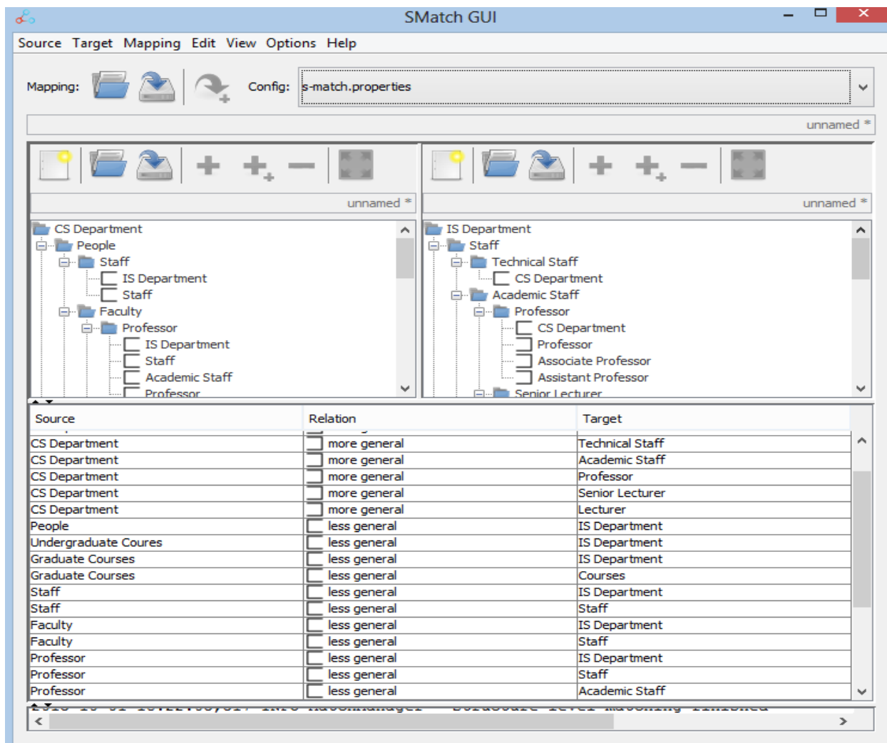
Figure 2. Default Matching Algorithm of S-Match (Too Permissive)
