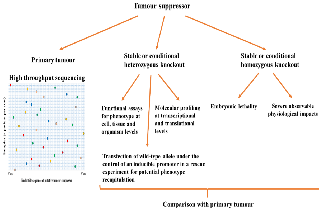
Figure 2. Intrinsic loss-of-function of tumour suppressor (TS) mutations complicates its identification and assignment of functional roles relative to oncogenic gain-of-function. Although lack of conserved signature in mutational profiles across patients is suggestive of a putative TS, functional characterization at the molecular and phenotypic levels are de rigueur for TS confirmation. Crucially, embryonic lethality of homozygous deletion of many TS (and lack of phenotypic data), meant that creation of stable or conditional heterozygous animal knockouts is a commonly used approach for phenotypic validation of a TS gene.
