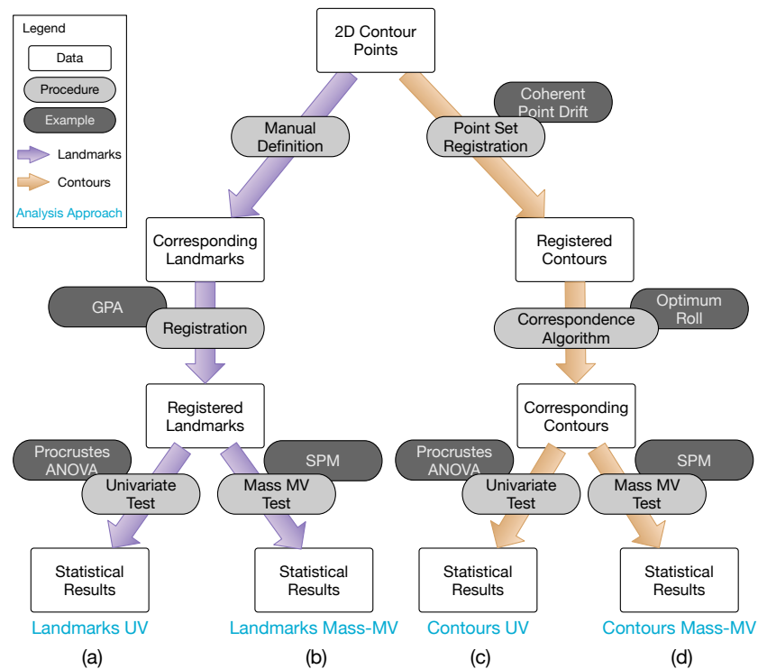
Figure 1 Overview of 2D contour data processing approaches employed in this paper. (A) The most common analysis approach, consisting of Generalized Procrustes Analysis (GPA) and Procrustes ANOVA for landmarks. (B) Same as (A), but using mass-multivariate (MV) analysis instead of Procrustes ANOVA's univariate (UV) approach. (C) and (D) are conceptually equivalent to (A) and (B), respectively, but operate on full contour data instead of landmark data, and can also be fully algorithmic. Statistical Parametric Mapping (SPM) is a methodology for mass-MV analysis of continuous data. See text for more details.
