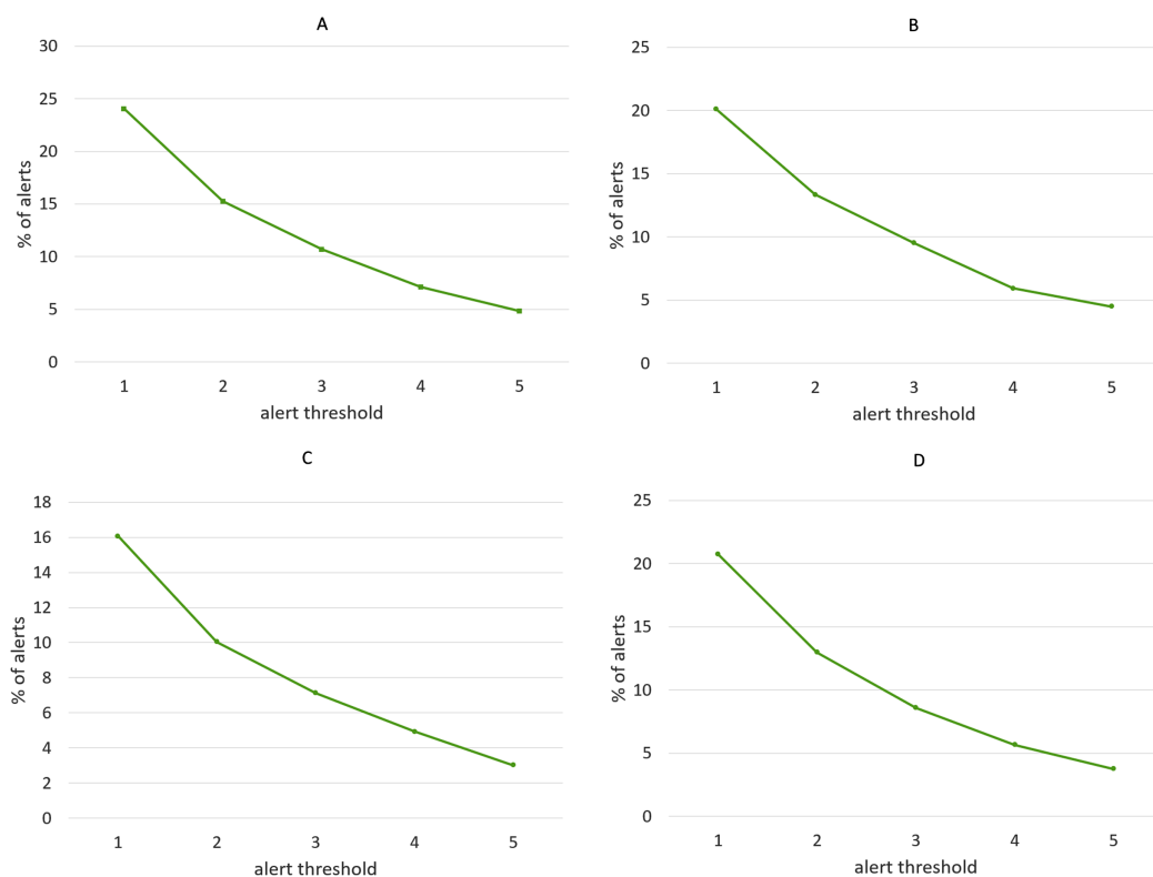
Figure 15 Percentage of alerts produced by the alert-generation algorithm in the time-span considered for the experiments (June 2016–March 2020), for different values of alert threshold. (A) Agglomerative. (B) K-Means. (C) K-Medians. (D) K-Medoids.
