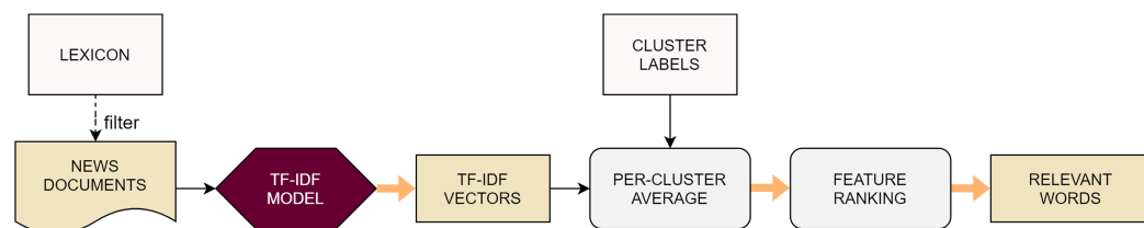
Figure 6 Flowchart of the algorithm used to extract the most relevant words from each cluster.
