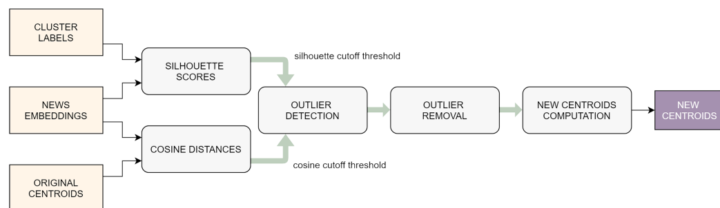
Figure 4 Flowchart of the outlier removal procedure. Full-size DOI: 10.7717/peerj-cs.438/fig-4
