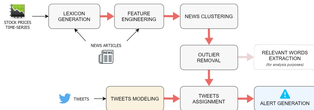
Figure 1 Overall architecture of the proposed approach. Full-size DOI: 10.7717/peerj-cs.438/fig-1
