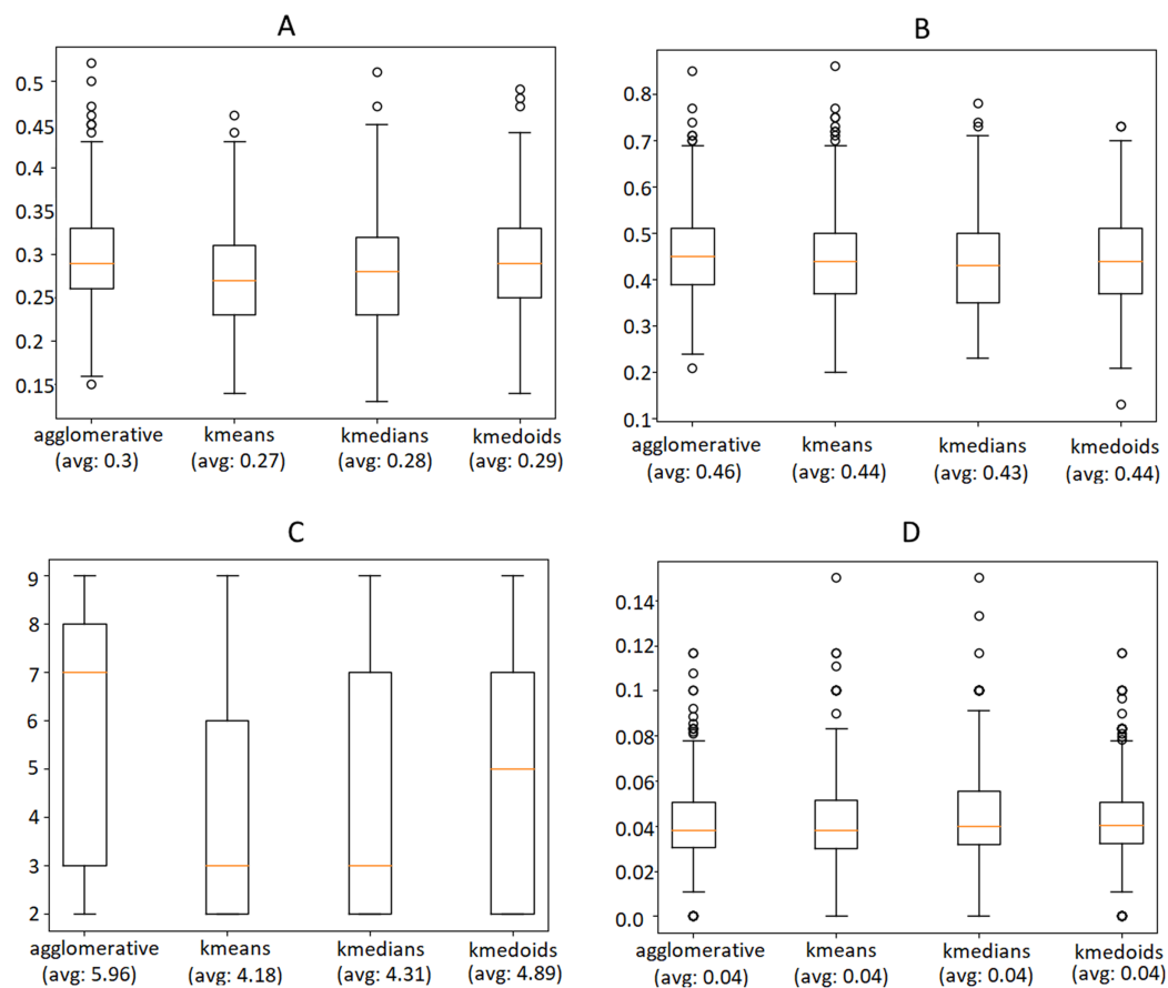
Figure 12 Comparison of the Silhouette Coefficient (A), Dunn Index (B), number of clusters (C) obtained by different clustering algorithms and overlapping between the clusters' relevant words (D). The horizontal orange line represents the median of the obtained scores whereas the average is indicated between parenthesis. For further details we refer the reader to the official documentation of matplotlib library: https://matplotlib.org/3.1.1/api/_as_gen/matplotlib.pyplot.boxplot.html .
