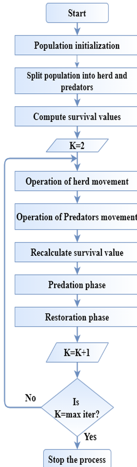
Figure 1 Flow diagram of SHO.
