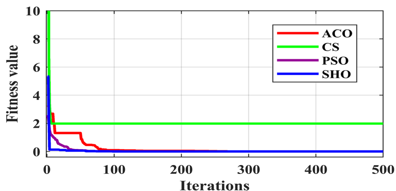
Figure 3 Comparison of convergence plot.
