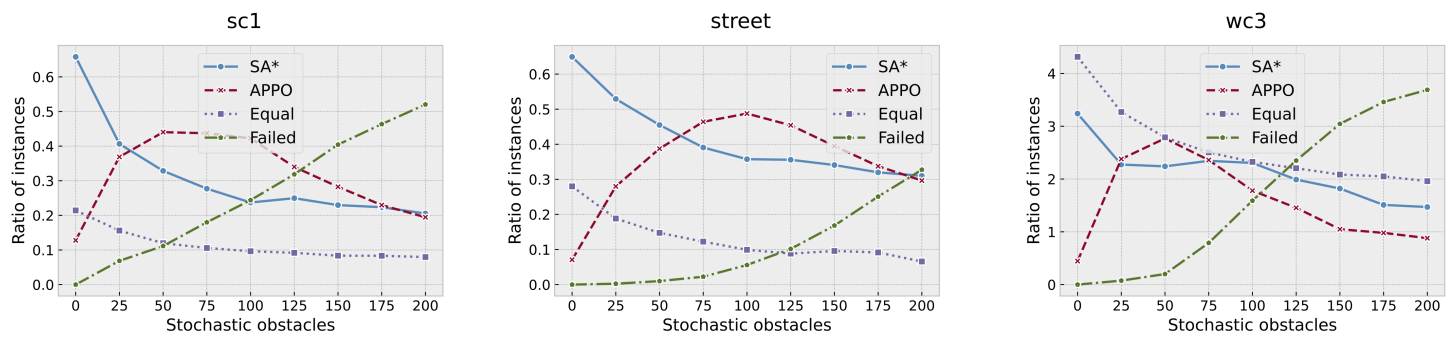
Figure 7 Comparison of the solutions found by SA* and APPO depending on the collection of the maps and number of stochastic obstacles. Points on “SA*” and “APPO” lines indicate the portions of instances for which the corresponding approach has found a solution of a better quality than other one. “Equal” correspond to the portion of instances for which both approaches have found solution with equal quality. “Failed” correspond to the portion of instances that were solved neither by SA* nor by APPO.
