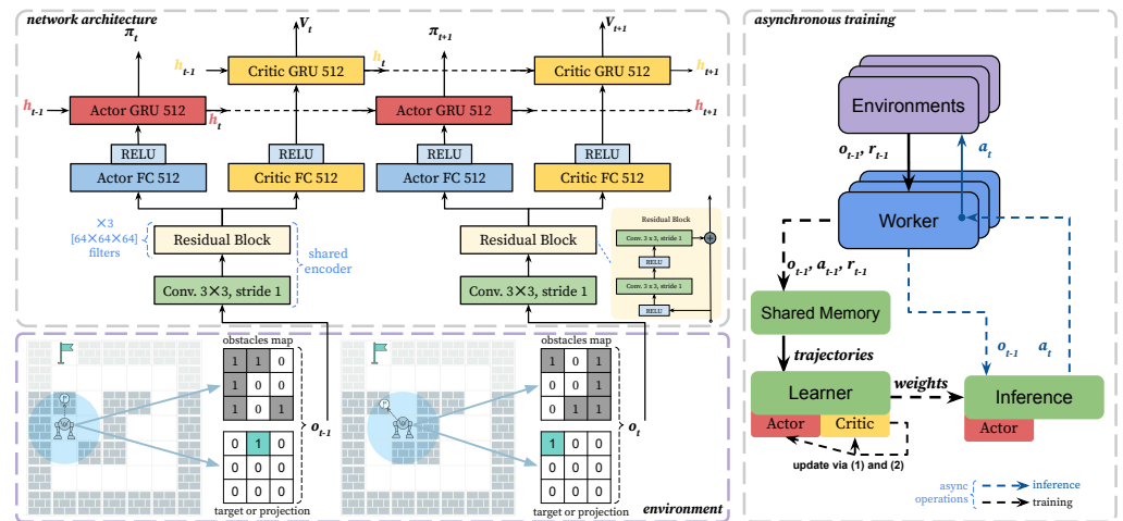
Figure 3 The scheme of the proposed asynchronous learning approach. The bottom-left part shows the environment and observation encoding. The top-left part of the scheme shows the neural network architecture. We use residual layers as a shared encoder and recurrent heads. The recurrent layers (GRU) are responsible for remembering obstacles and environment dynamics. The right part shows the asynchronous learning procedure. The green blocks show GPU computations.
