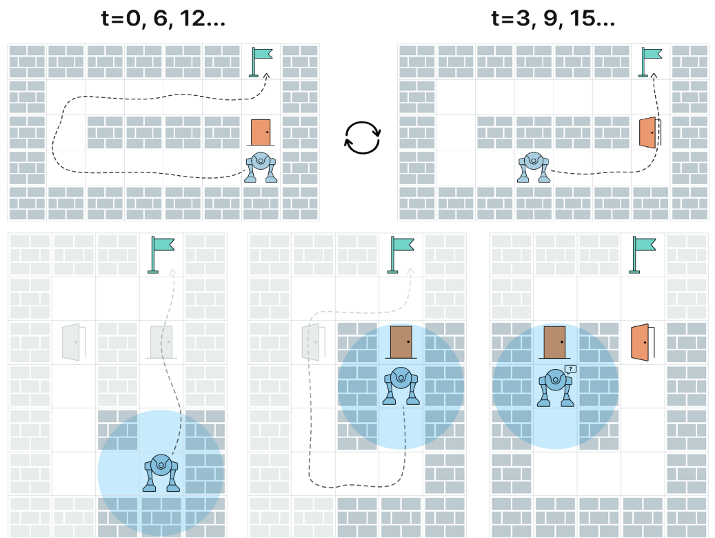
Figure 1 The challenges associated with pathfinding in stochastic environments. Top row: the robot with unlimited field of view is stuck in an oscillating behavior due to blocking/unblocking of a single grid cell (which might correspond to opening/closing the door by humans). Bottom row: due to the partial observability the robot is unaware that the previously blocked cell becomes traversable (the door opens) and, thus, the robot is not able to plan a path to the goal. Both cases can be successfully solved by the learnable policy suggested in the paper, which is empirically shown to learn such behaviors as “wait for an obstacle to disappear,” “keep exploring the environment for additional options of reaching the goal”, etc.
