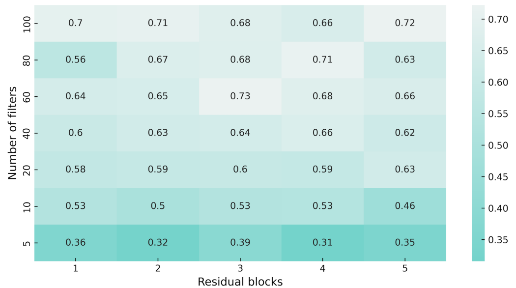
Figure 5 Heatmap of the network architecture parameters. We used a version with 60 filters and three residual blocks as encoder in APPO model for all experiments, since it showed better performance in our hyperparameter sweep.
