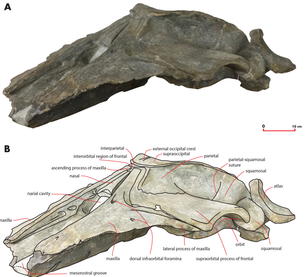
Figure 5 The holotype skull in anterolateral view. Anterolateral view of the left side of the holotype skull of Nehalaennia devossi (NMR 999100014035). (A) Photographic representation. (B) Interpretation. Scale bar equals 10 cm.
