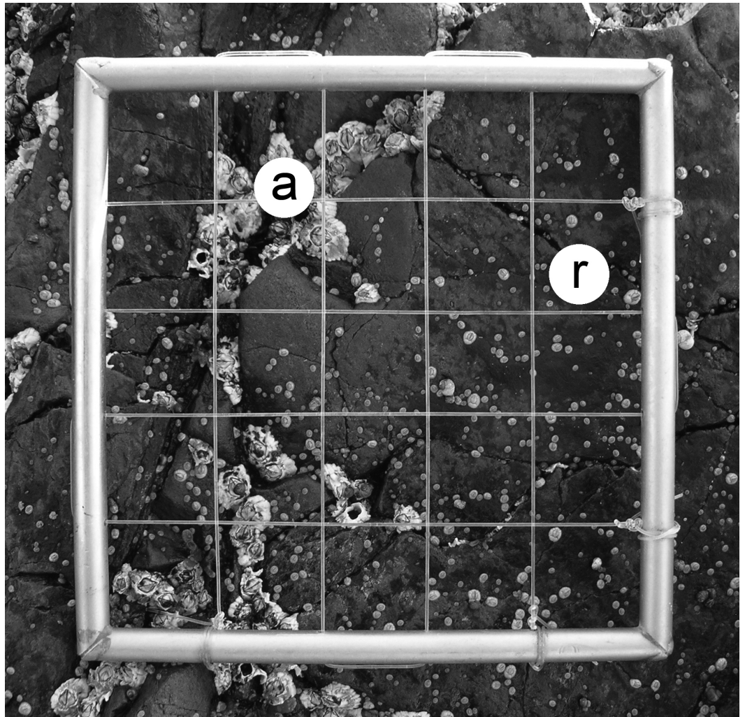
Figure 1 Typical view of a wave-exposed, high-intertidal habitat on the Gulf of St. Lawrence coast of Nova Scotia in June, showing barnacle adults (a) and recruits (r). The sampling quadrat is 10 cm × 10 cm. Photograph by RA Scrosati.
