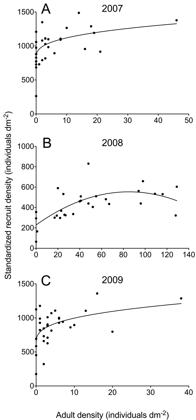
Figure 2 Relationships between standardized barnacle recruit density (scaled to the available area for recruitment in each quadrat) and the density of pre-existing adult barnacles (always scaled to quadrat area) in June 2007 (A), 2008 (B), and 2009 (C) for wave-exposed, high-intertidal habitats on the Gulf of St. Lawrence coast of Nova Scotia. Each graph shows the model that best describes the adult–recruit relationship (see Table 1 for model parameters).
