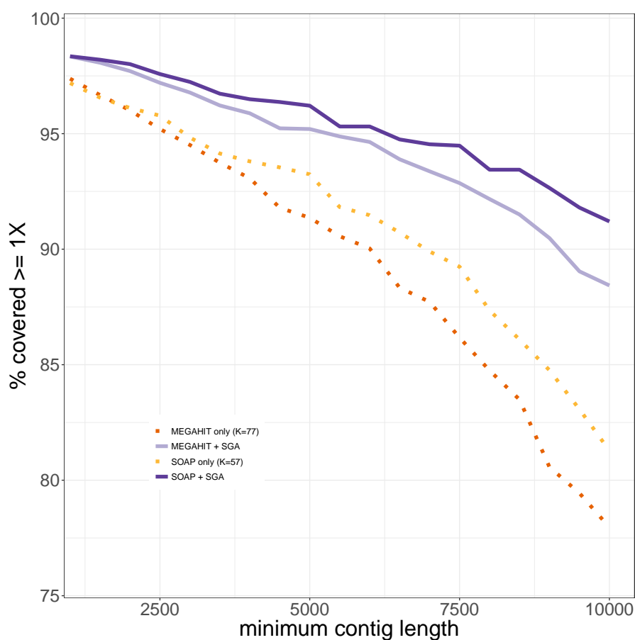
Figure 4 The percentage of the reference genome of Mycobacterium leprae TN that could be covered using only contigs longer than the minimum contig length. Results from the first and second layer assemblies are shown.
