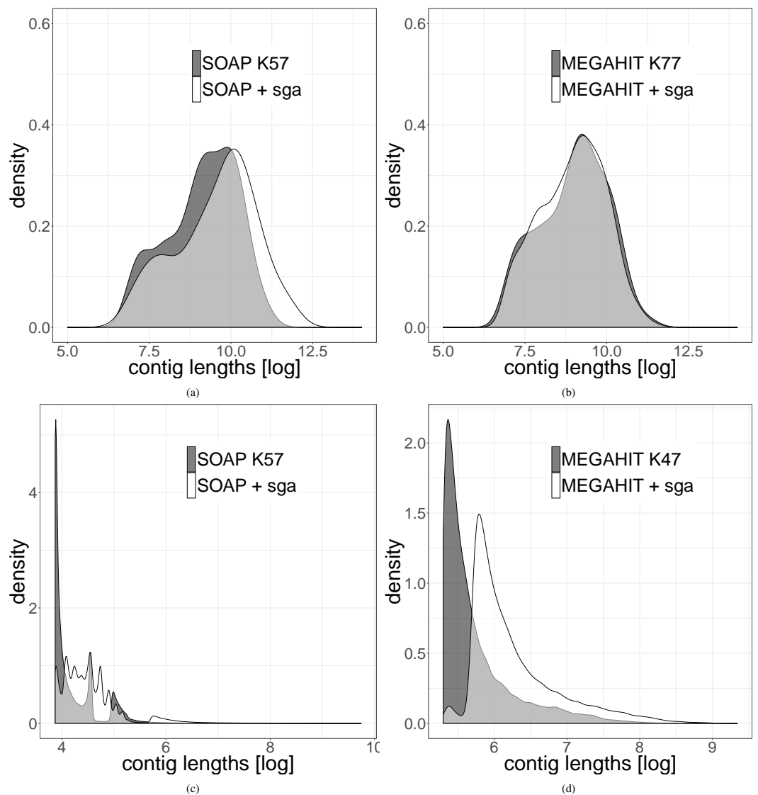
Figure 3 Distribution of the length of the contigs generated by the different assemblies. The results generated by the second layer assembly with SGA are shown in white. The results of one first layer assembly is shown in dark grey. The light grey part represents the overlap of both methods. (A) Shows the results using SOAPdenovo2 in the first layer and (B) shows the results using MEGAHIT in this layer for the leprosy data. (C and D) Show the same results on the pestis data. In order to highlight the differences, the data were logarithmized.
