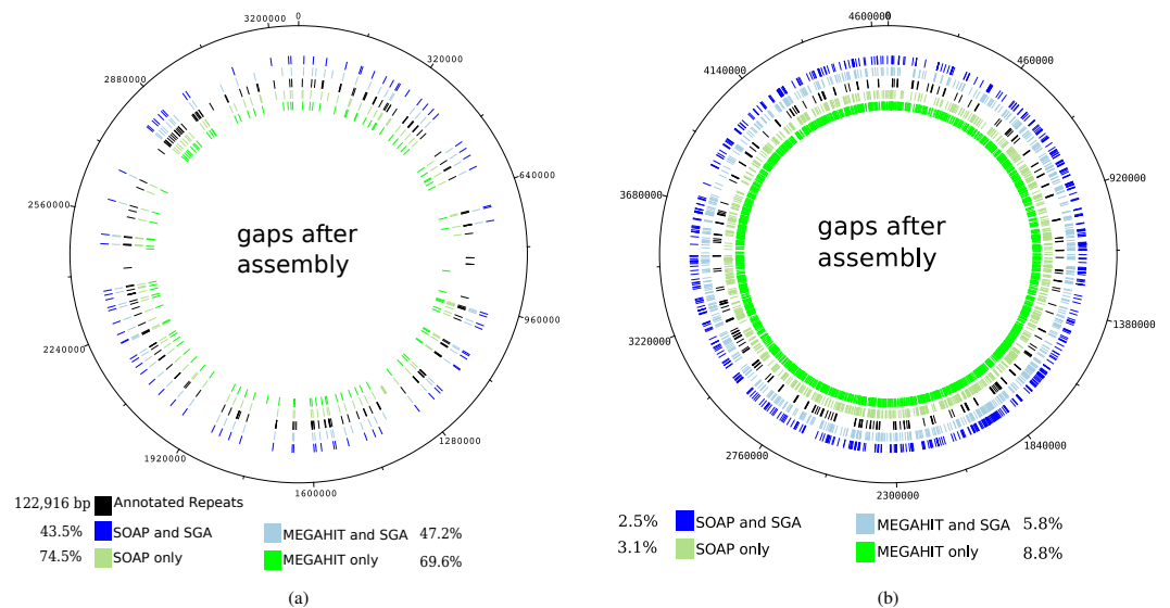
Figure 5 Gaps in the mapping of the contigs against the reference genome of Mycobacterium leprae TN (A) and Yersinia pestis CO 92 (B) together with annotated repeat regions in the respective reference genome. The outer ring represents the gaps that occur after the mapping of the contigs that were generated by the second layer assembly with SGA after a first layer assembly with SOAPdenovo2. The second outer ring shows the same but for a first layer assembly using MEGAHIT. The middle ring represents the annotated repeat regions of the reference genome. The second inner and innermost ring represent the gaps after using the best individual SOAPdenovo2 and MEGAHIT assemblies, respectively. The percentages represent the relative number of unresolved bases in annotated repeat regions for Mycobacterium leprae (in total 122,916 bp). For Yersinia pestis , the respective values represent the percentage of unresolved genomic positions.
