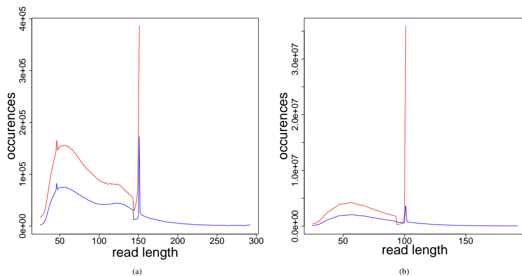
Figure 2 Read length distribution for the different preprocessed (adapter clipped and quality trimmed) fastq files for (A) Jorgen625 ( Mycobacterium leprae ) and (B) OBS137 ( Yersinia pestis ). Red, unmerged reads; blue, reads after merging.
