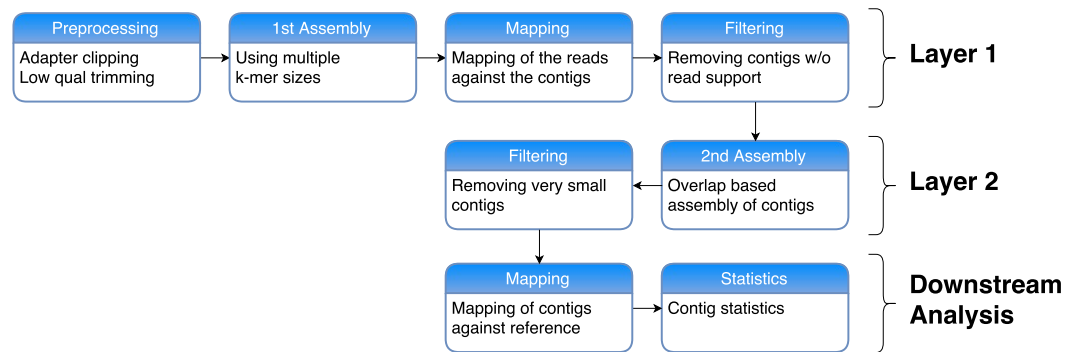
Figure 1 Workflow of our two-layer assembly approach. First the reads are preprocessed by removing sequenced adapters and clipping low-quality bases. After that, multiple de novo assemblies are generated using a de Bruijn graph approach with multiple values for k . The reads are then mapped back against each of these resulting contigs and the contigs with no read support are filtered out. In Layer 2, these filtered contigs are then combined and assembled again using an Overlap-Layout-Consensus approach. Very short contigs are removed. The resulting contigs are mapped against a reference genome and contig statistics are calculated in order to assess the quality of the assembly.
