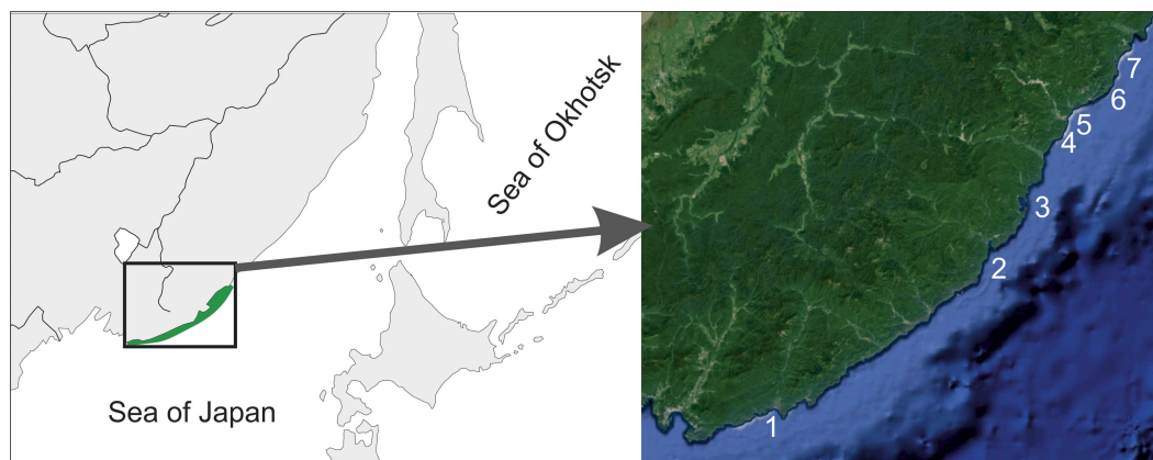
Figure 1 Surveied area map. 1–Kievka Bay (42.84°N 133.65°E), 2–Olga Bay (43.74°N 135.27°E), 3–Vladimir Bay (43.91°N 135.50°E), 4–Dva Brata, Senkina Shapka (44.33°N 135.84°E), 5–Rudnaya Bay, Brynner Cape (44.36°N 135.80°E), 6–Tretya Langou, Kamenka Bay (44.42°N 135.94°E), 7–Oprichnik Bay (44.45°N 136.00°E).
