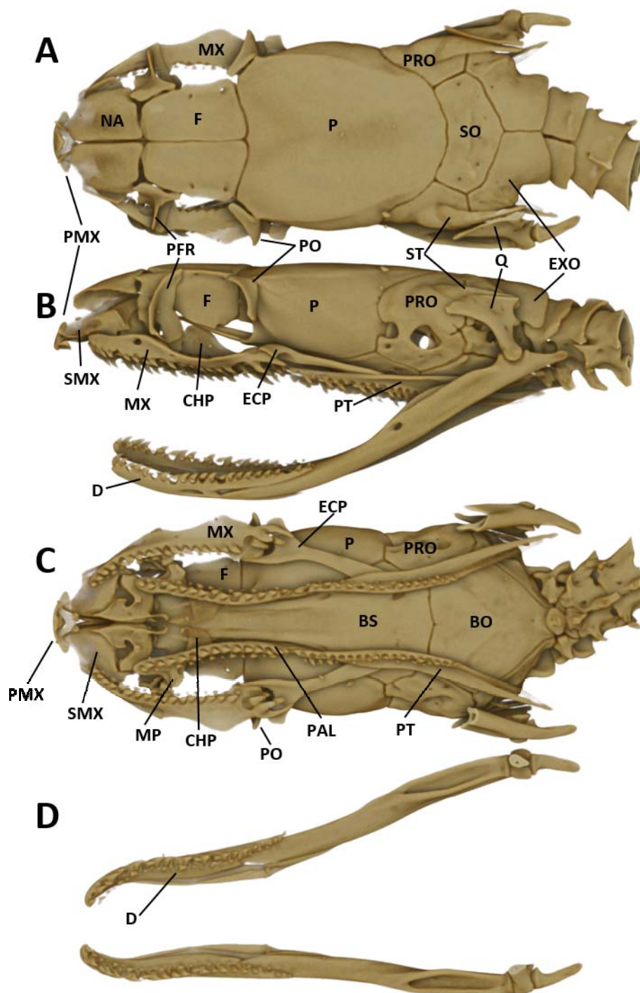
Figure 5. Micro-CT images of the male paratype of Tantilla tjiasmantoi sp. nov. from La Libertad: dorsal (A), lateral (B), and ventral views of the skull (C, lower jaw removed), and dorsal view of lower jaw (D). See Materials and Methods section for explanation of the abbreviations of the skull structures.
