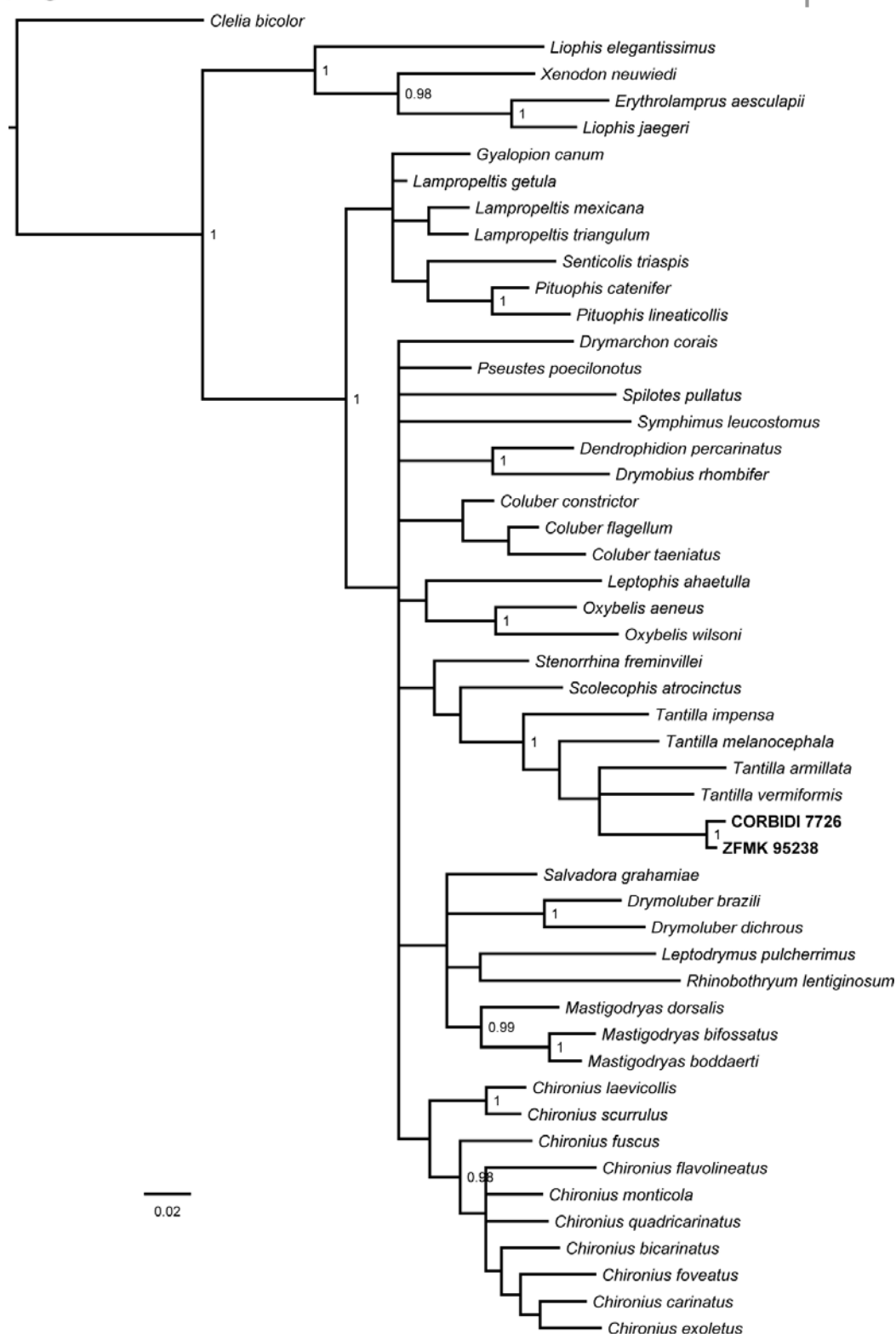
Figure 1. Bayesian consensus tree based on 788 bp of mitochondrial DNA (12S and 16S rRNA) of our specimens (CORBIDI 7726 and ZFMK 95238) and 48 further species representing 27 genera of American colubrid snakes. Numbers at nodes are the Bayesian posterior probabilities (values < 0.95 not shown).
