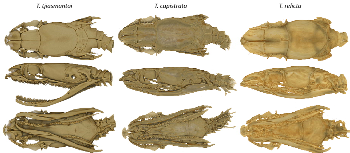
Figure 6. Micro-CT images of the dorsal (above), lateral (center), and ventral (below) views of the skull of three species of Tantilla : T. tjiasmantoi sp. nov. from Peru (left), T. capistrata from Lambayeque, Peru (ZFMK 85028, middle), and T. relictta from Florida, USA (ZFMK 84387, right).
