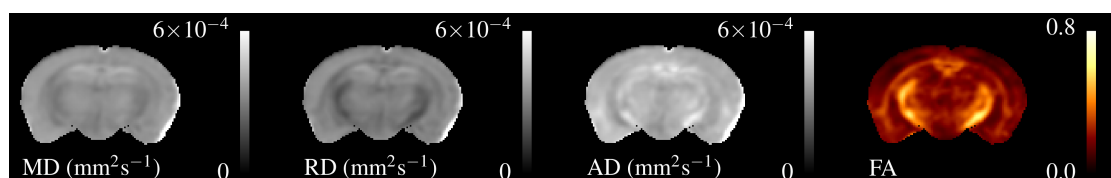
Figure 3. Single subject maps of the four DTI parameters - Mean, Radial and Axial Diffusivity and Fractional Anisotropy. These have lower resolution than the relaxometry data but the WM tracts are still visible. MD, AD & RD all show similar contrast, but the absolute value of AD is higher than RD.
