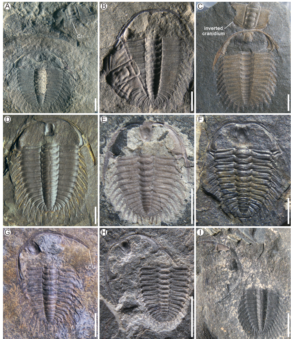
Figure 3 Examples of Henningsmoen's configuration in Oryctocephalus indicus from the Cambrian Kaili Formation of Guizhou Province, South China. (A–C) Types I shows the preservation of cranidium (Cr); (B) Except for the cranidium is internal surface, the rest of the structures are external surface. (C) Shows the cranidium inverted before the LCU. (D–F) Types II shows the lower cephalic unit (LCU) nearly in situ and the displaced cranidium is missing; (G–I) Types III shows the laterally rotated of the LCU and the displaced cranidium is missing. Specimen Nos: A, GTBM17-1866; B, GTBM9-3-3706; C, GTBM16-437; D, GTBM9-3-3745; E, GTBM9-2-4282; F, GTBM9-5-4029; G, GTBM9-5-4110; H, GTBM8-5-832; I, GTBM9-3-2110. All scale bars are two mm.
