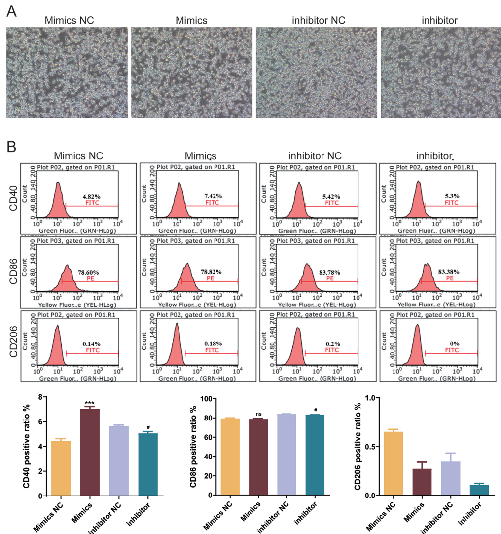
Figure 6 Effects of mmu-miR-146a-5p on microglial conversion. (A) Cell morphology diagram of BV-2 cells transfected with mmu-miR-146a-5p mimics or inhibitors. (B) Expression of CD40, CD86, and CD206 in BV-2 cells transfected with mmu-miR-146a-5p mimics or inhibitors. *** P < 0.001 vs. Mimics NC groups; # P < 0.05 vs. inhibitor NC groups. ns: no significance.
