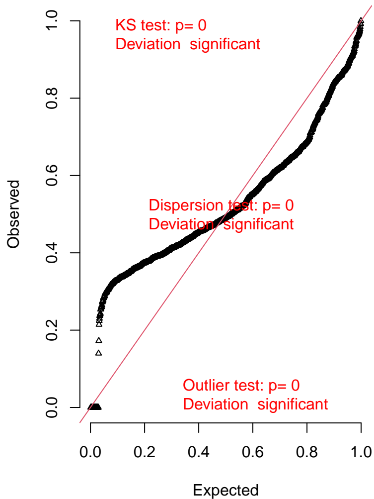
QQ plot residuals
