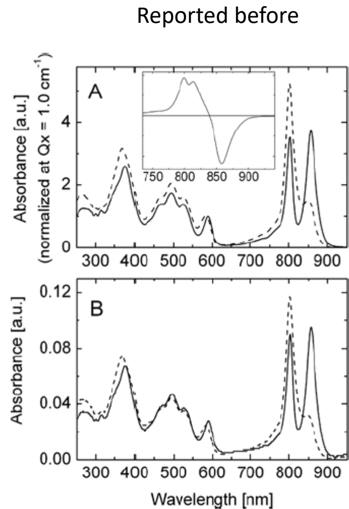
Figure 3 Room temperature absorption spectra of HL (continuous line) and LL (broken line) LH2 complexes from Rps. palustris 2.1.6. (A) in solution and from (B) dissolved crystals
