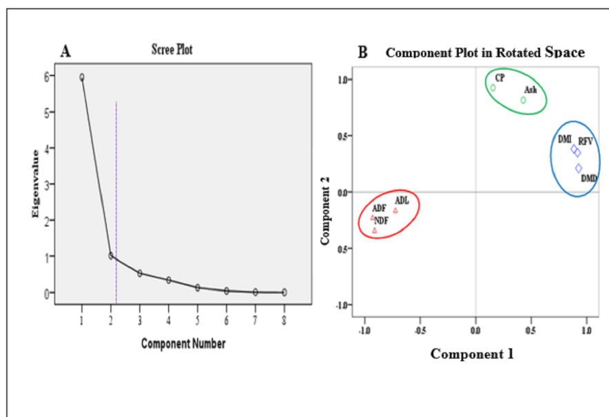
Figure 5 Scree plot: Eigenvalues plotted in descending order (A) and Principal Components in a two-dimensional space (B).
