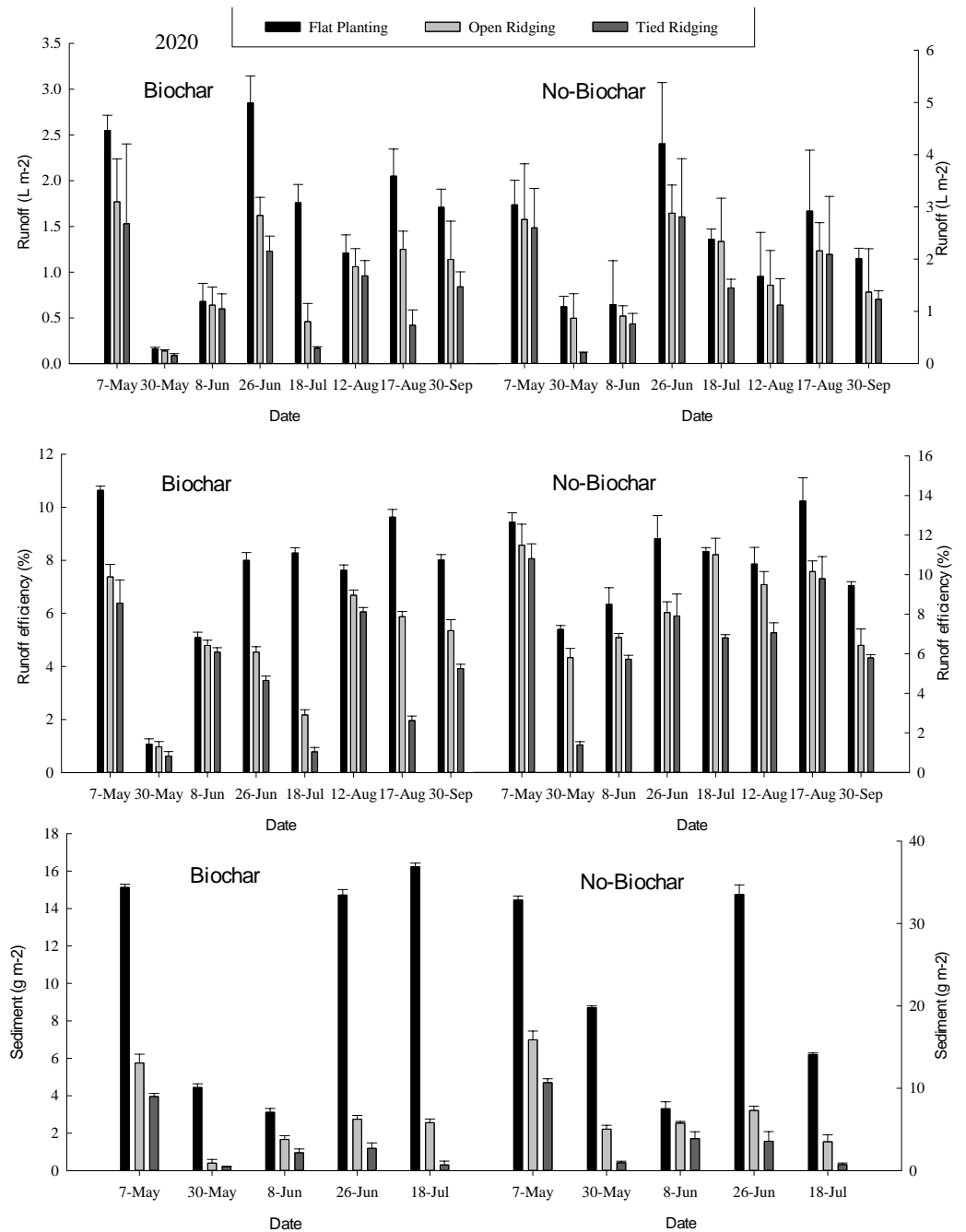
Figure 5 Runoff, runoff efficiency and sediment in different treatments. The means (columns) labeled with the same letters within each category are not significantly different at the 5% level (Tukey's-b test ANOVA).
