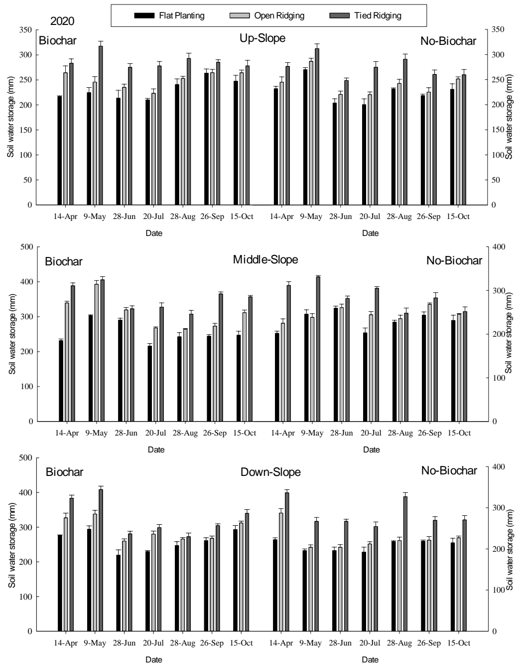
Figure 7 Soil water storage in furrows in 0–200 cm soil depth in various treatments. The means (columns) labeled with the same letters within each group are not significantly different at the 5% level (Tukey's-b test ANOVA).
