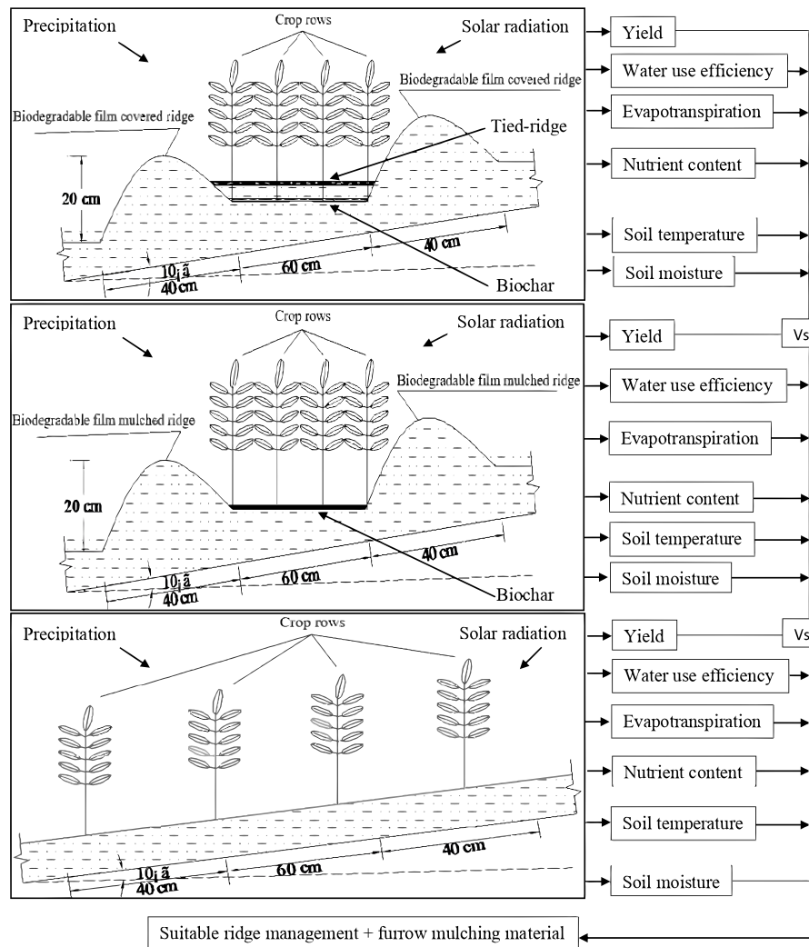
Figure 3 Schematic diagram for alfalfa production in rainwater harvesting system with biochar amendment on sloping land.
