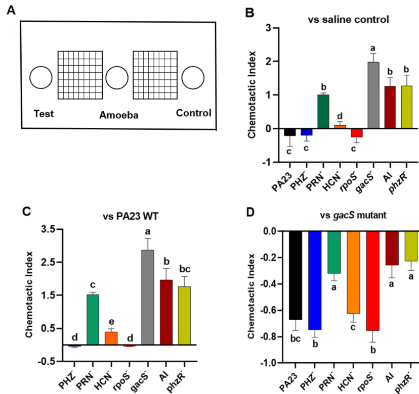
Figure 5 Chemotactic response of Acanthamoeba castellanii towards PA23 WT and derivative strains. (A) Schematic diagram illustrating Petri plate set up. Active amoebae were placed in the center well; the test bacterium was placed in the test well, and PA23 WT, the gacS mutant or saline was added to the control well. Chemotactic preference assays were carried out against saline control (B), PA23 WT (C), and the gacS mutant (D). The chemotactic response was determined as follows: the number of amoebae migrating towards the test well/the number of amoebae migrating towards the control well. Values > 0 indicated attraction; values < 0 indicated repellent activity. Assays were performed in triplicate and the experiment was repeated three times. Error bars indicate \pm SD; columns labelled with the same letter do not differ significantly by the Tukey test ( P > 0.05 ).
