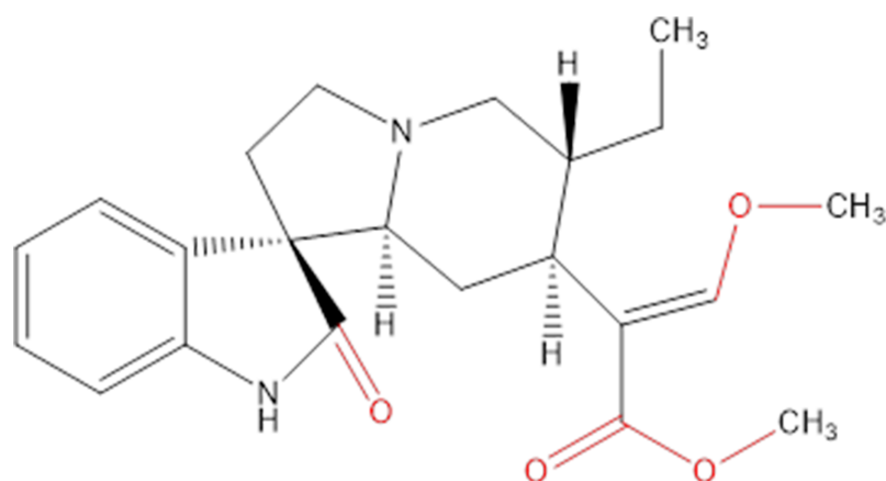
Figure 1 Chemical structure of hirsutine (MW = 368.47).
