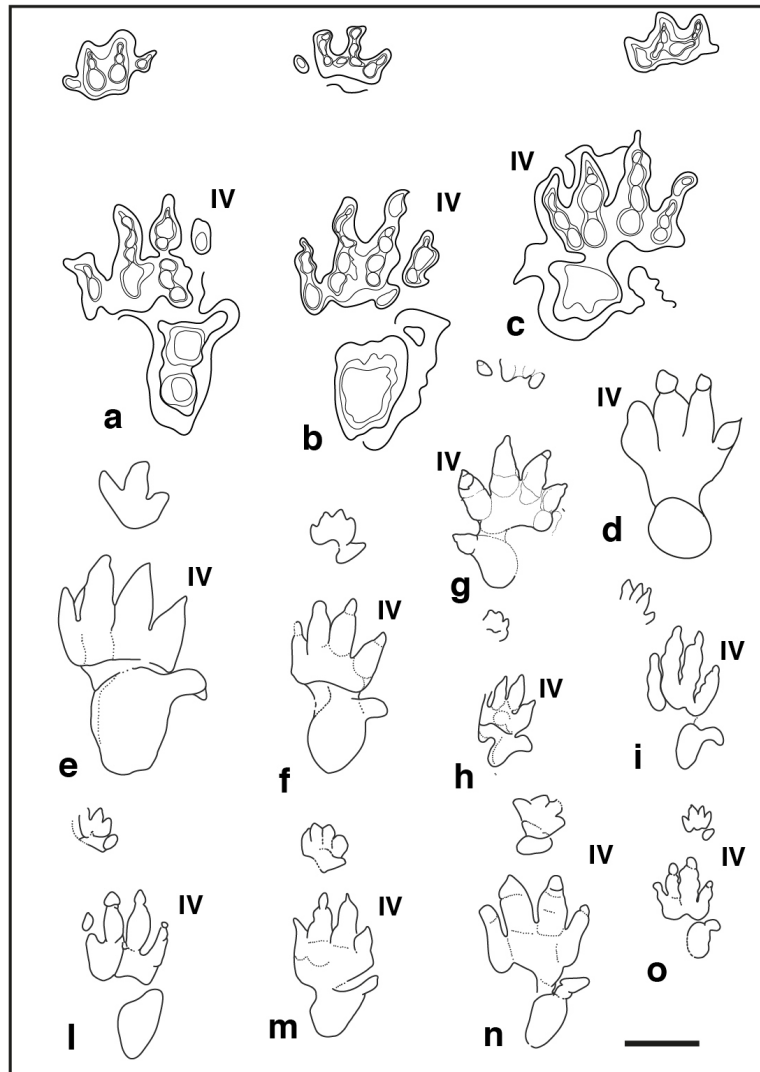
Figure 8 Pentadactyl tracks from the Lower and Middle Triassic, assigned to the ichnogenus Isochirotherium and their comparison with the studied tracks of the Gardetta ichnospite: (A), (B), (C), pes manus sets of the GT-7 trackway; (D) GT-3 isolated pes imprints of the lower track surface; (E) Isochirotherium herculis pes manus set from the “Thüringischer Chirotheriensandstein” (Lower Triassic), Germany; (F) Isochirotherium marshalli pes manus set from the Holbrook Member of the Moenkopi Formation (Middle Triassic), Penzance, Northern Arizona; (G) Isochirotherium infernense manus pes set from the Middle Triassic (late Anisian) of Adige Valley, Bolzano, Italy; (H) Isochirotherium coltoni pes manus set from the Wupatki Member of the Moenkopi Formation (Lower Triassic), Meteor Crater, Arizona; (I) Isochirotherium lomasi pes manus set from the Middle Triassic (Anisian) of Cheshire, Great Britain; (L) Isochirotherium coureli pes manus set from the Middle Triassic (Anisian-Ladinian) of the Massif Central, France; (M) Isochirotherium hessbergense pes manus set from the “Thüringischer Chirotheriensandstein” (Lower Triassic), Germany; (N) Isochirotherium demathieui pes manus set from the Middle Triassic of Mont d’Or Lyonnais, France; (O) Isochirotherium soergeli pes manus set from the “Thüringischer Chirotheriensandstein” (Lower Triassic), Germany. Scale bar 10 cm.
